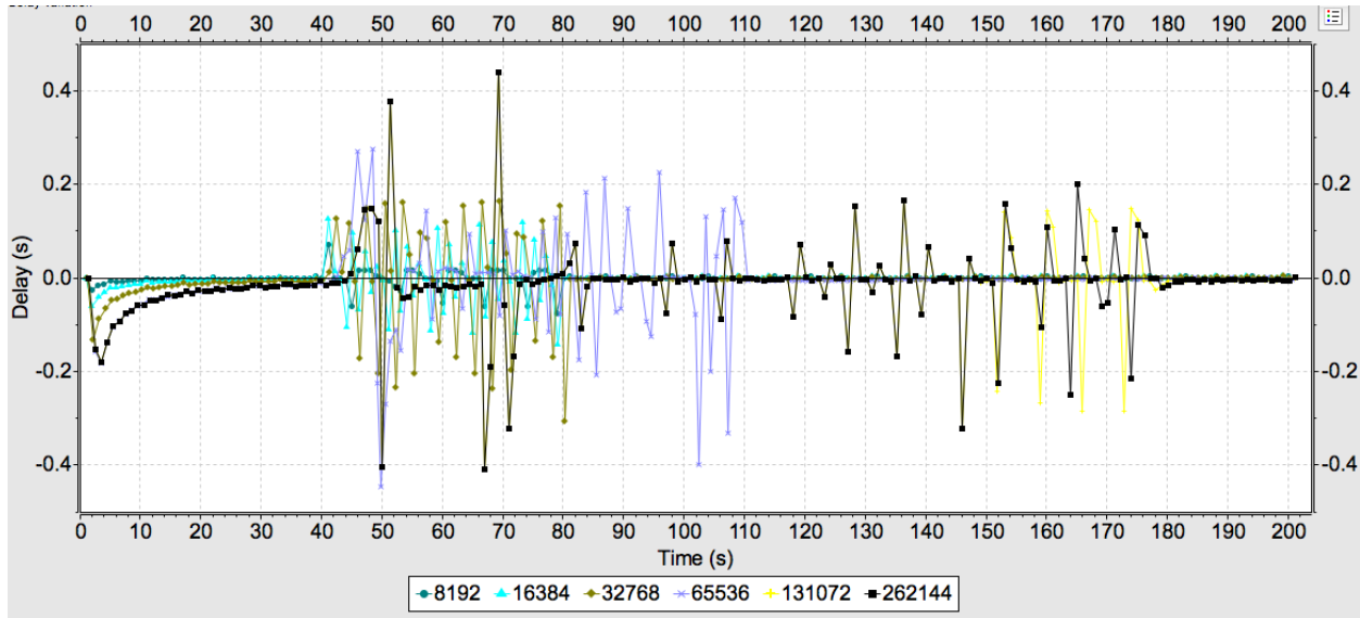
Figure 4: Packet Delay Variation for varying Advertised Window sizes
