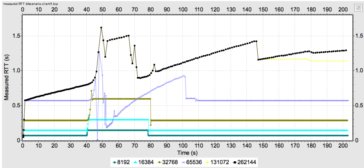
Figure 3: Measured RTT for varying Advertised Window sizes
