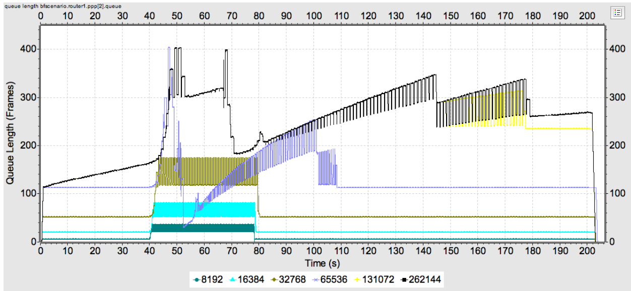
Figure 2: Queue Length for varying Advertised Window sizes
