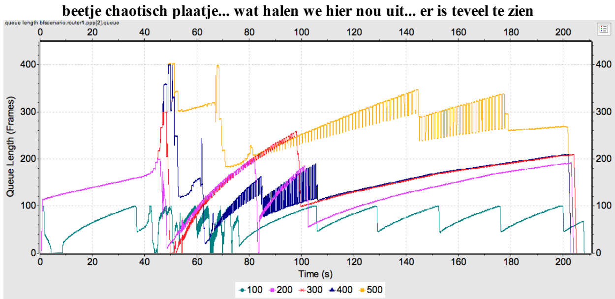
Figure 7: Queue Lengths for varying Buffer Size
