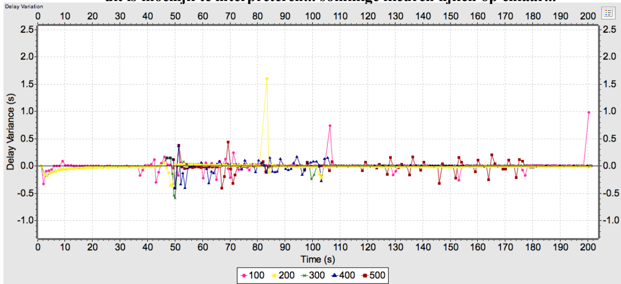
Figure 5: Packet Delay Variance for varying Buffer Size
