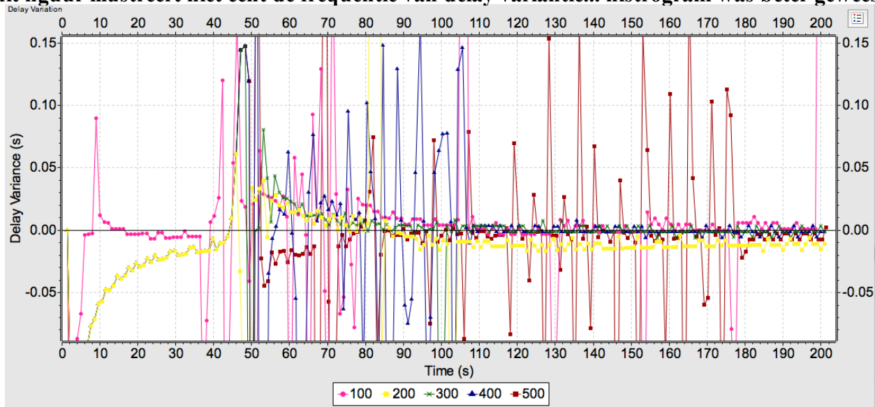
Figure 6: Packet Delay Variance for varying Buffer Size (zoomed)
