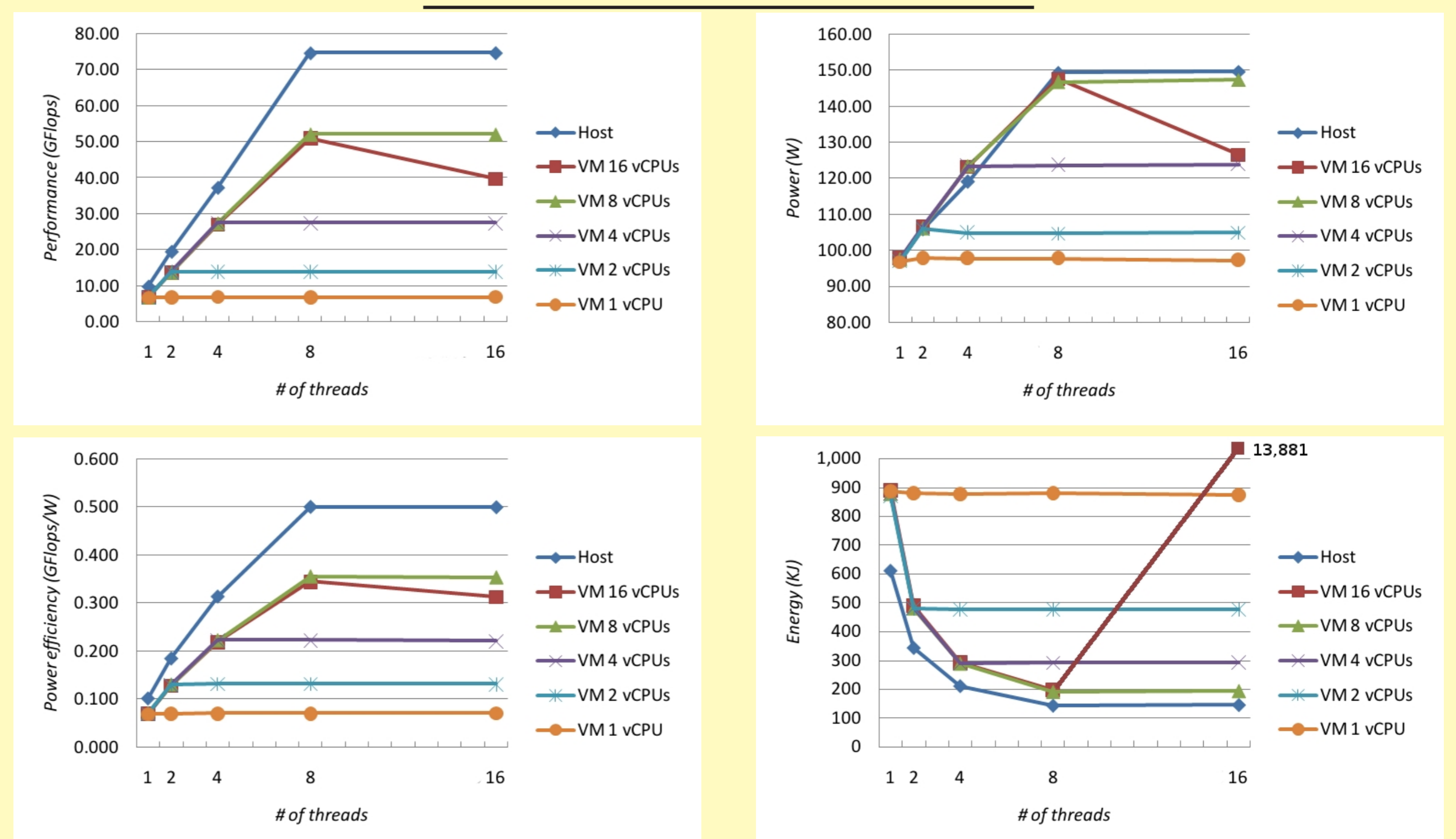
Fig. 2. Several VMs with the same configurations except the number of vCPUs.
