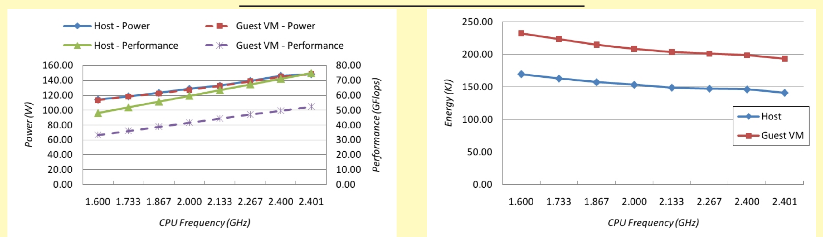
Fig. 1. Performance, power and energy consumption of LINPACK benchmark for various CPU frequencies.
